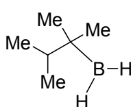
Thexil borano
